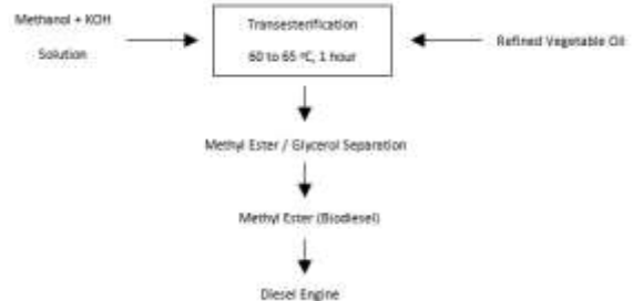
Figure 1. Procedure of manufacturing biodiesel through transesterification with vegetable oil
