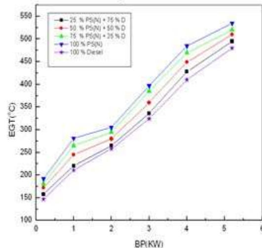
Fig. 3 Shows the variation of Exhaust Gas temperature with Brake power output for Palm Stearin oil and its blends with diesel in the test engine. 25% blend of Palm stearin has lower EGT compared to all other blends for all loads.
