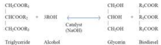
Transesterification reaction
